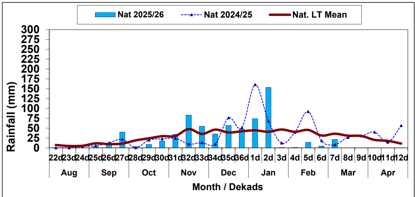
Figure 1: Rainfall distribution 1 st dekad March 2026
