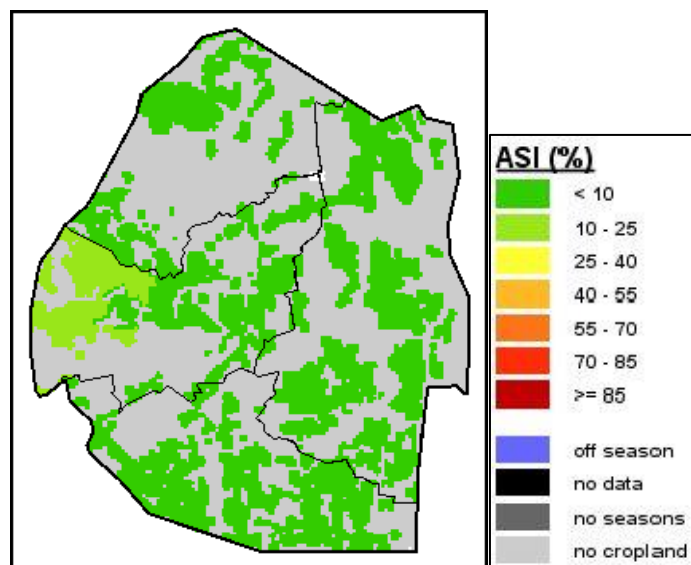
Image 1: Agriculture Stress Index 1 st dekad March 2026 Source: FAO-GIEWS
