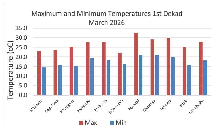
Figure 2: Maximum and Minimum temperatures 1 st dekad of March 2026
