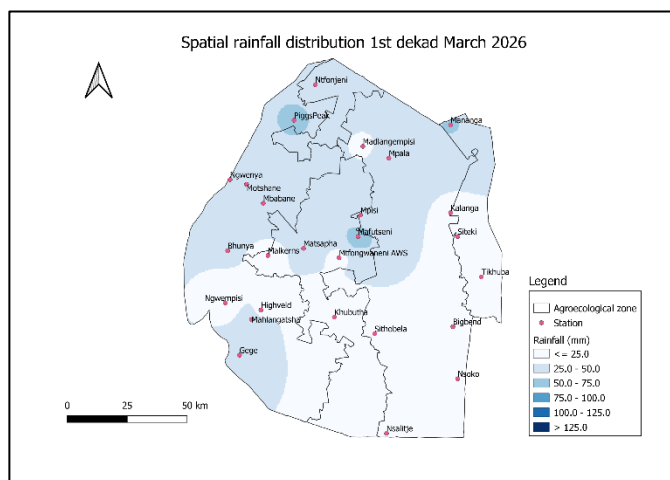
Map 1: Spatial rainfall distribution 1 st dekad March 2026
