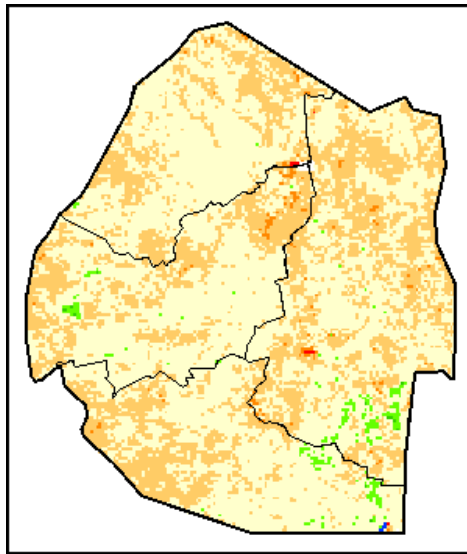
Image 2: Normalized Difference Vegetation Index (NDVI) Anomaly (1 st Dekad March 2026) Source: FAO-GIEWS
