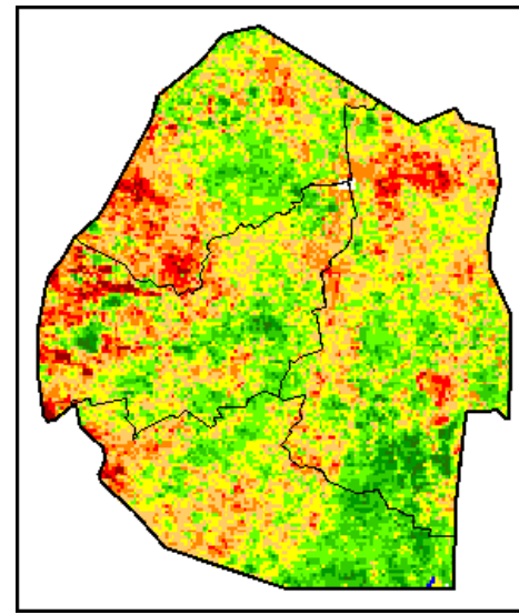
Image 3: Vegetation Health Index (VHI) (1 st Dekad March 2026) Source: FAO-GIEWS
